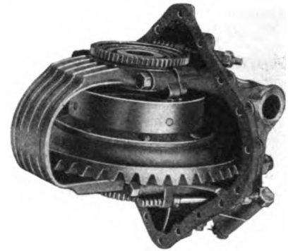
TIMKEN DIFFERENTIAL AND BEVEL CARRIER.
